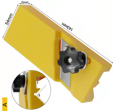
45 degree trimmer
